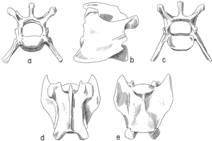
FIG. 15. — Lumbar vertebra, a. anterior, b. lateral, c. posterior, d. dorsal, e. ventral, x 2. Based on Tavolara-Ty. 8746, Ty. 7777.
