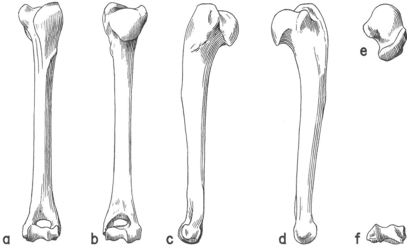
FIG. 19. — Left humerus, a. dorsal, b. posterior, c. lateral, d. medial, e. proximal, f. distal, x 1\frac{1}{2} . Based on : Tavolara-Ty. 8776, Ty. 8780, Ty. 8788.
