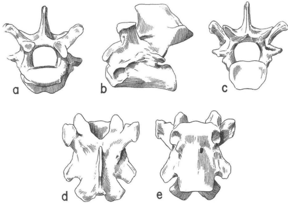
FIG. 14. — Thoracic vertebra, a. anterior, b. lateral, c. posterior, d. dorsal, e. ventral, x 2. Based on Tavolara — Ty. 7782, Ty 7784.
