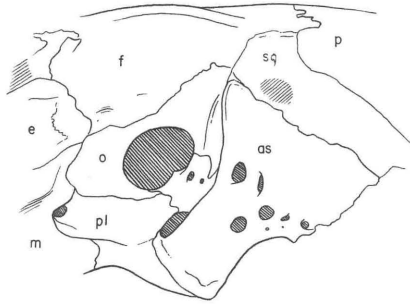
FIG. 3. — Lateral view of left orbit, zygoma removed, x 2. as — alisphenoid, e — ethmoid (?), f — frontal, m — maxilla, o — orbitosphenoid, p — parietal, pl — palatine, sq — squamosal.
