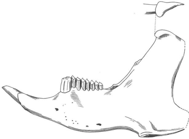
FIG. 6. — Lateral view of jaw and dorsal view of condyle, x 2. Composite jaw of figs. 6-7 based on: Monte San Giovanni-Br. 359, Br. 363.
