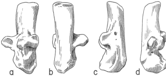
FIG. 31. — Left calcaneum, a. anterior, b. posterior, c. lateral, d. medial, x 3. Based on specimens from Monte San Giovanni.
