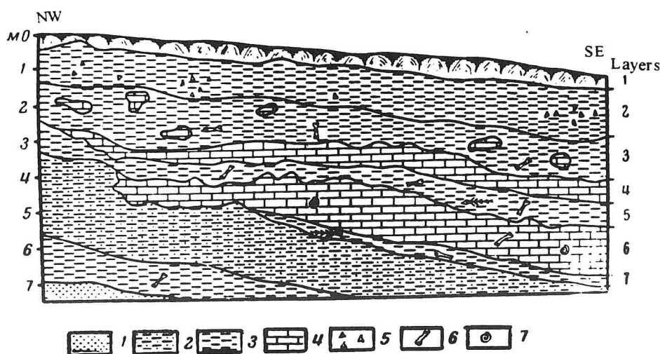
Figure 2.— Geological section of the Tagai outcrop (Logachev et al. , 1964). 1: sand; 2: sandy clay; 3: clay; 4: limestone; 5: rubble; 6: mammalian remains; 7: mollusks.
