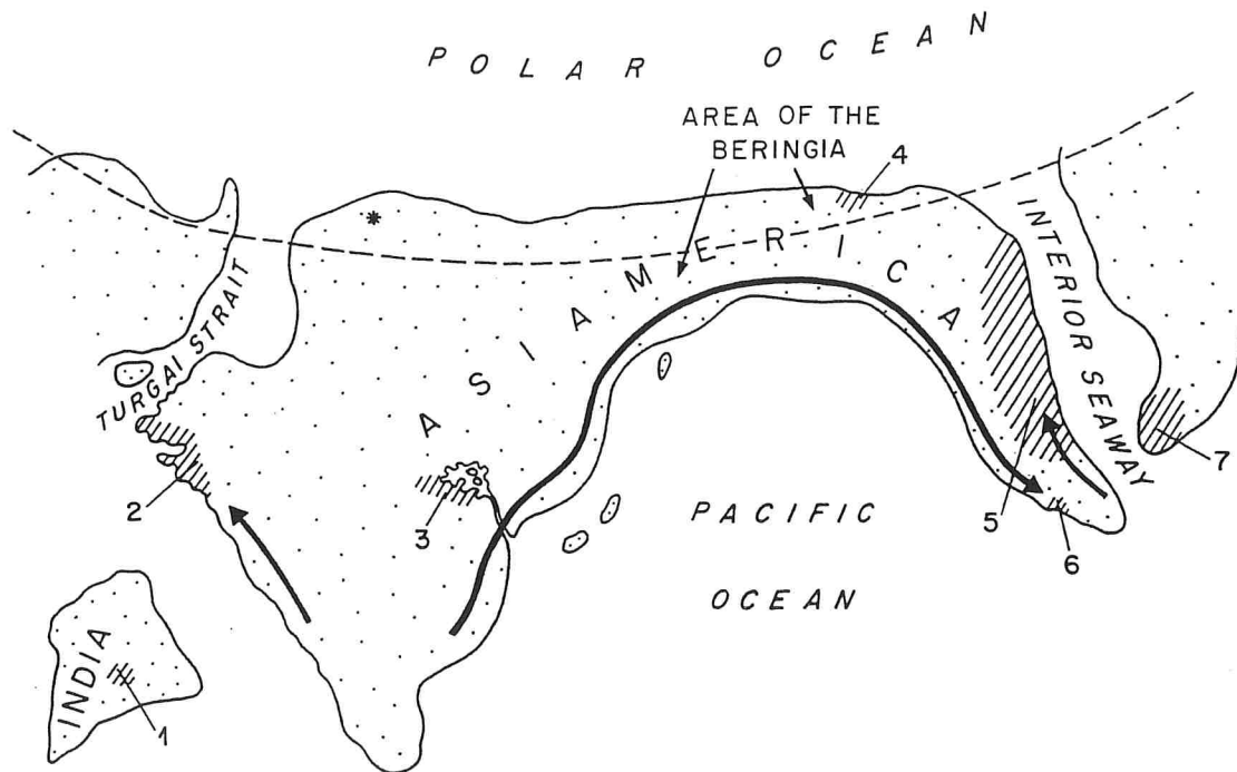
Figure 3.— Very simplified outline of Asiamerica and adjacent lands of the Northern Hemisphere, showing localities with mammalian remains and the principal migrational routes of advanced eutherians during the Late Cretaceous.
