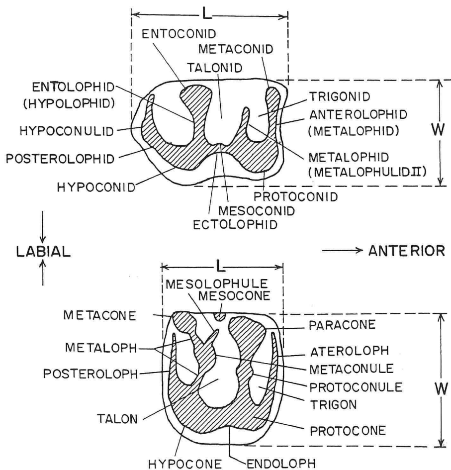
Fig. 4.— Idealized chapattimyid upper and lower molars depicting the dental terminology and method of measurements of teeth.
