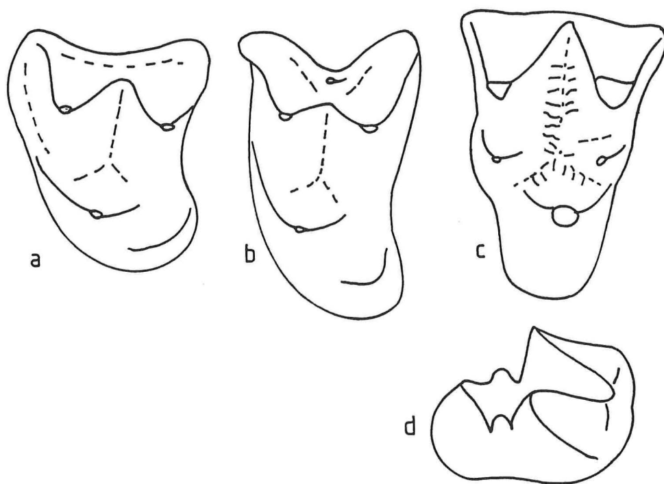
Figure 4.— Left upper molars in which crests of the paracone and metacone are straight, and the mesostyle is not involved. a-c in partially lingual view. a , Ageina (primitive chiropteran); b , Scotophilus (chiropteran with secondarily reduced hypoconid); c , Cynopterus volans (dermopteran). d , Cynocephalus variegatus (dermopteran), posterior view.
