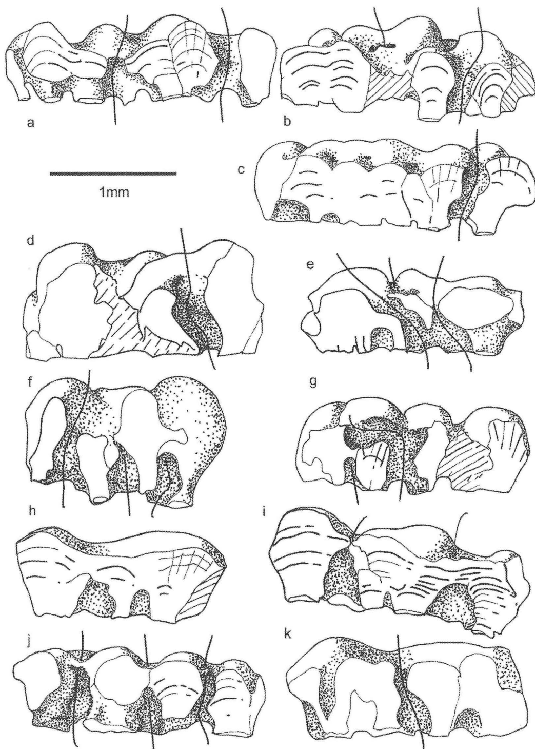
Figure 3.— Broken radial surfaces of fragments of Pseudomegaloolithus atlasi oogen. nov. oospec. nov., showing the organization of the units and the prolatocanaliculate pore canal system; from Achloulj 2 locality, level 18-19 (Middle Atlas, Morocco). a: ACH2-211; b: ACH2-213; c: ACH2-216; d: ACH2-220; e: ACH2-223; f: ACH2-224; g: ACH2-225; h,i: ACH2-227; j: ACH2-228; k: ACH2-237. The black lines indicate the course of the pore canals.
