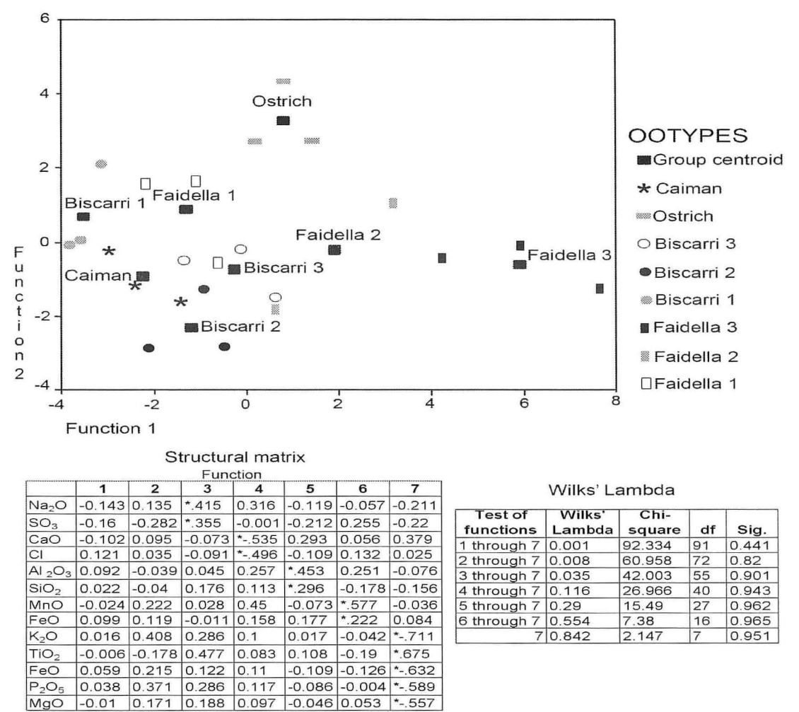
Figure 3.— Factorial discriminant analyses and structural matrix. Ootypes are from caiman, ostrich and Megaloolithus siruguei from Faidella and Biscarri. Ootypes show no significant difference when Function 1 is plotted against Function 2. Asterisk in structural matrix represents the strongest correlation between each variable and any discriminant function. The strongest correlation of Na and S occurs with function 3 (see also text). Seven functions have been used in the discriminant analysis. The Wilk's Lambda table represents the test of functions. Significance < 0.10 indicates that group means differ.
