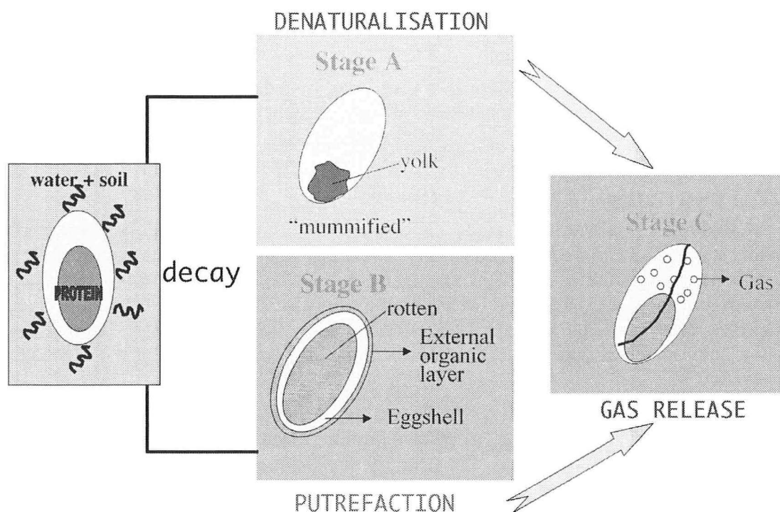
Figure 1.— Schema showing the model of an egg depicted as a protein pouch enclosed in a permeable but continuous hard matrix. Egg alterations are based mainly on protein denaturation with an additional role played by the eggshell. The initial stage involves the release of organic matter and subsequently two different paths can be follow: A- "mummified" eggs (denatured proteins) and B- "rotten eggs" (decay and autolysis). The final stage is characterized by gas release as a by-product of denaturalisation and putrefaction.
